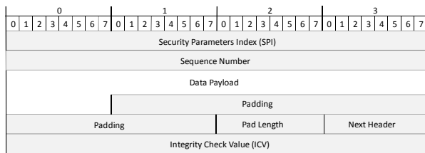
Fig. 10: IPsec ESP header
