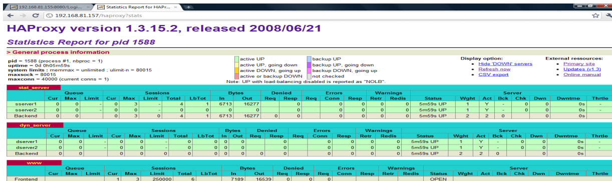
Figure 2: HAProxy Statistics
