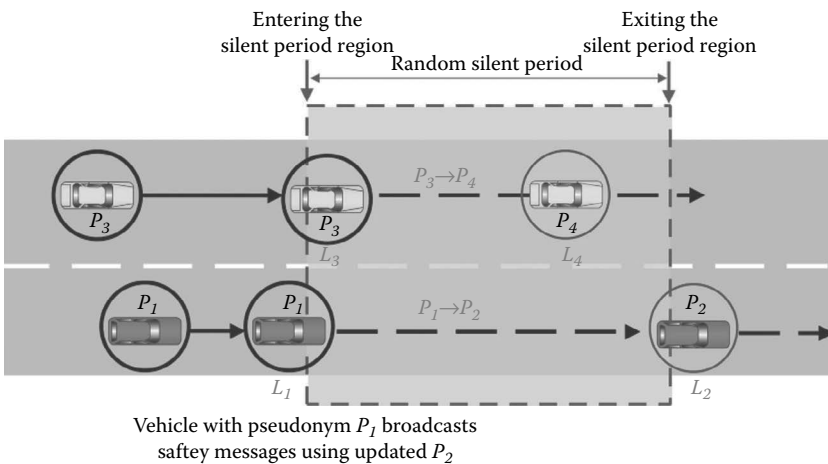
Figure 8.3: The illustration of silent period scheme.
