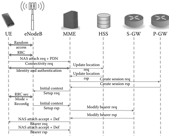
Figure 20.2: NAS attach signaling procedure.
