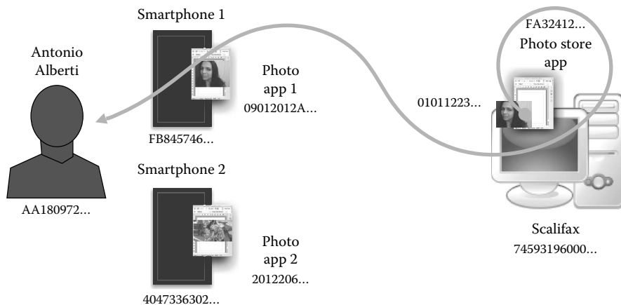
Figure 11.9: Provenance can be determined by decrypting SVN backward from the subscriber service up to the original content publisher. For instance, the SVN “01011223...” of the female picture can be bound to the SVN “FA32412...” of the “Photo store app.” By resolving this name binding, an authorized entity can determine the provenance and integrity of the exchanged data. This approach can be allied to the established SLAs among services, enabling the creation a trustable fellowship of “things,” representative software in the IoT context.
