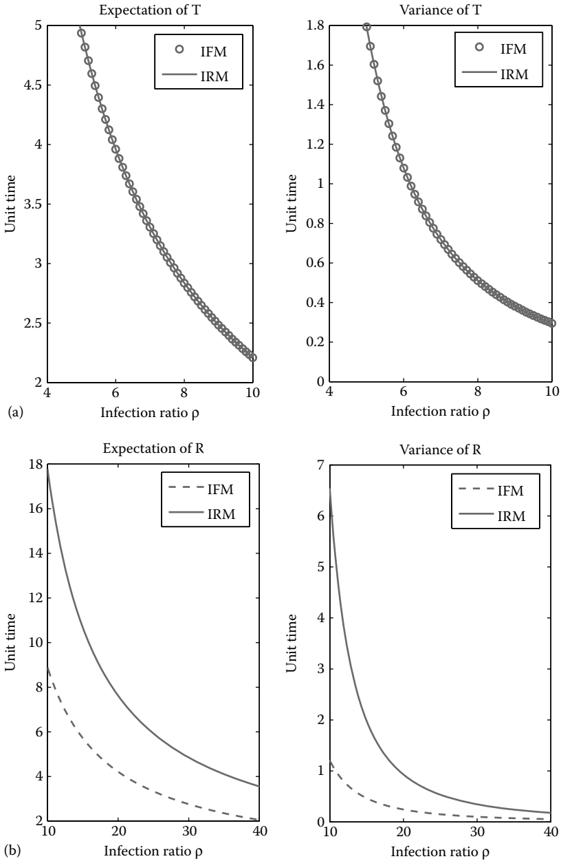
Figure 4.6: Numerical results of incubation period T and remaining lifetime R in feasible regions. (a) Expectation and variance of T . (b) Expectation and variance of R .
